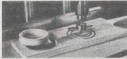
◀ Fly cutter is used here for a double cut to create a wooden ring. Be careful at breakthrough for the ring will be free in the hole.
